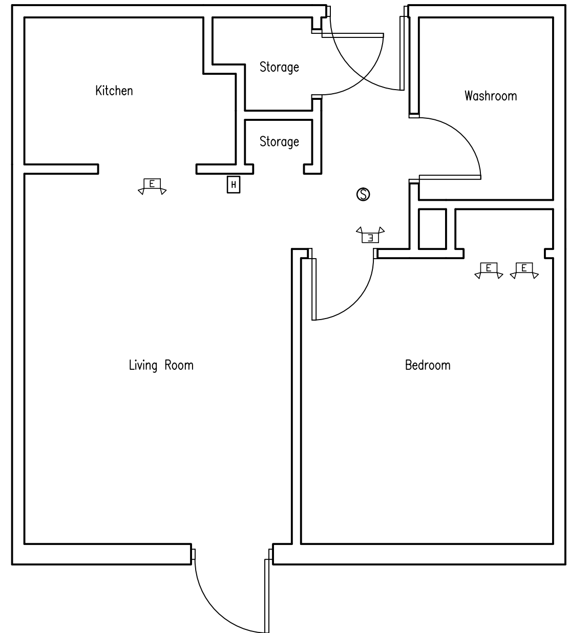
2 Typical Hearing Impaired Suite 1/4" = 1'-0"
