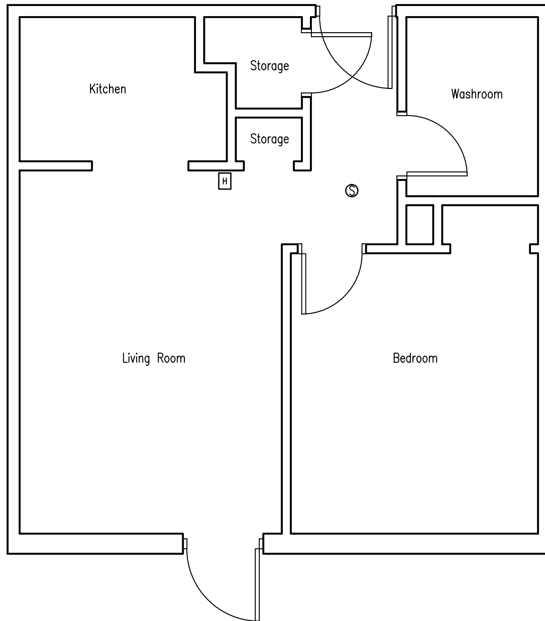
1 Typical Suite 1/4" = 1'-0"
